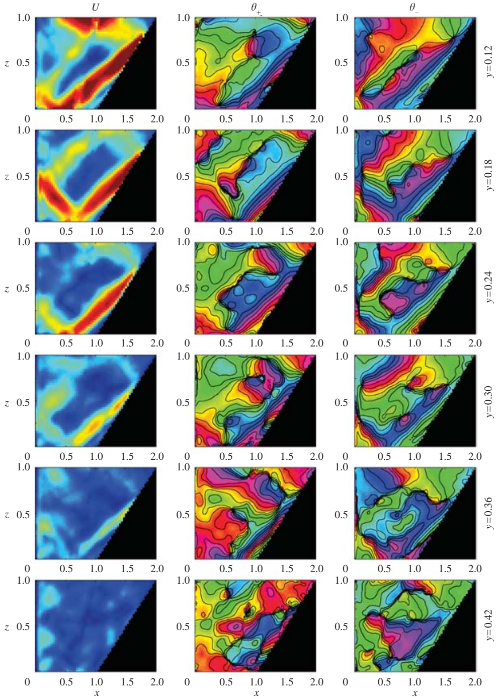
FIGURE 11. Ellipse parameters U , \theta_+ and \theta_- for the self-similar attractor at y=0.12 , y=0.18 , y=0.24 , y=0.3 , y=0.36 and y=0.42 . The scale for U ranges from 0 to 0.4 \text{ cm s}^{-1} .
